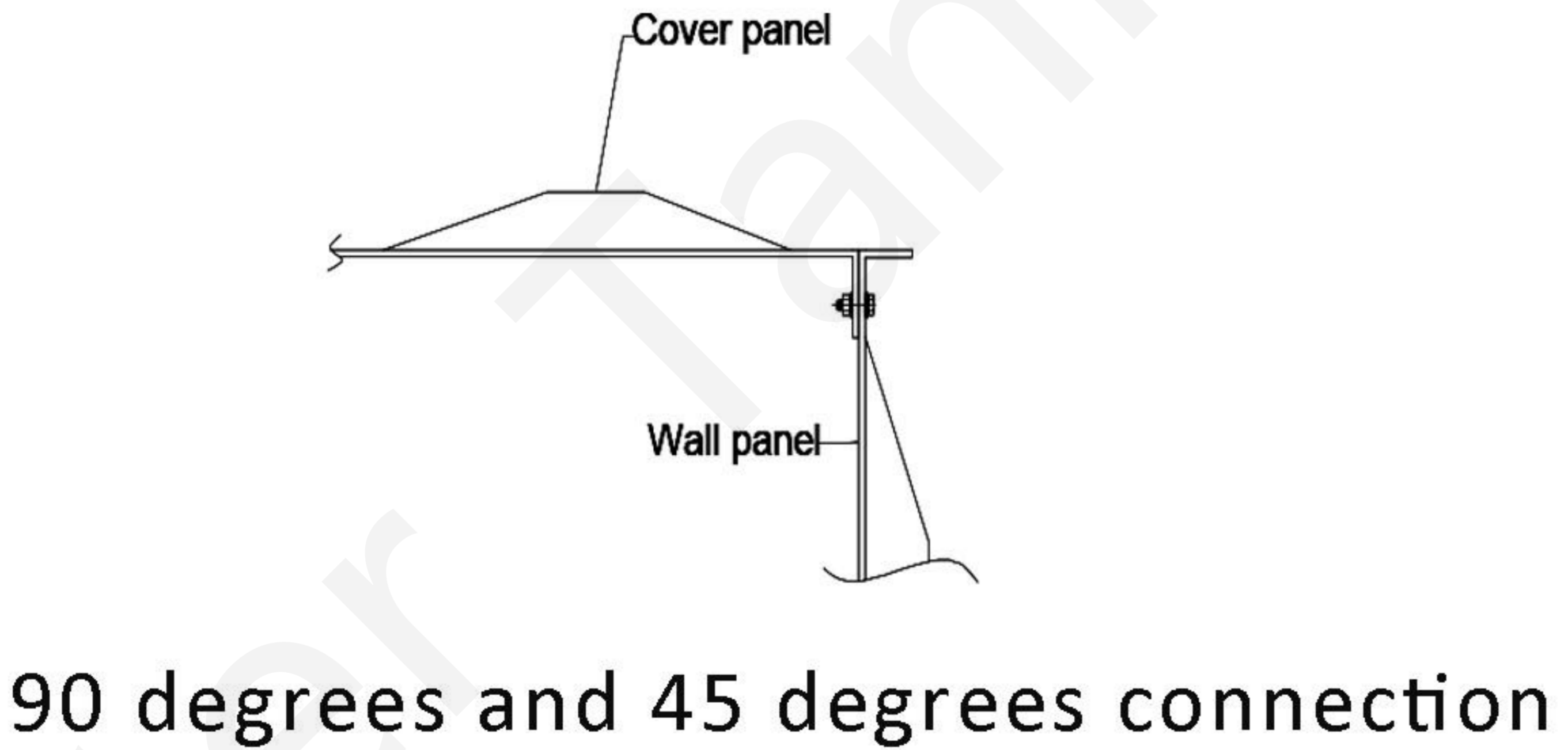
Side panel and Roof panel
